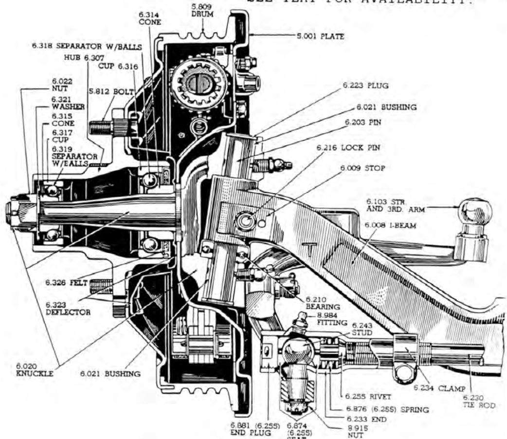
FRONT AXLE—CONVENTIONAL TRUCK (EXC. H.VY. DUTY)
