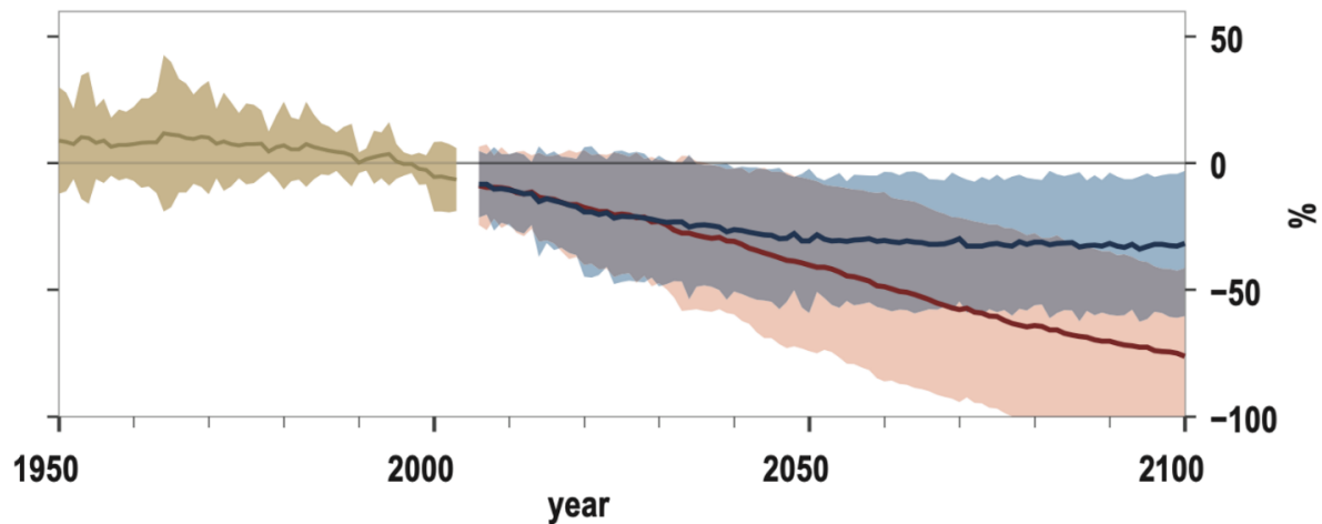
Figure 23. Projected permafrost areal change (x-axis) of the topmost 3 m until 2100
