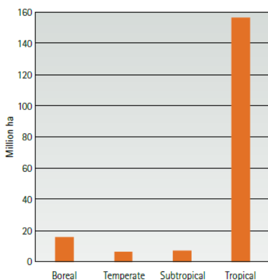
Figure 8. Estimated area with partial canopy-cover loss by climatic domain between 2000 and 2012 (FAO, 2015)
