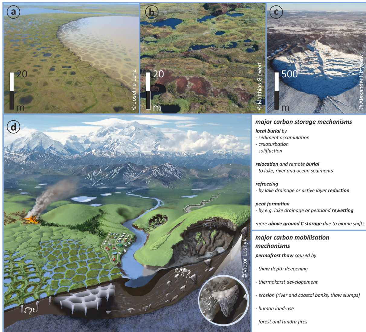
Figure 24. Permafrost degrades as the ice in the ground melts in response to e.g. climate warming, human disturbance, or more wildfires
