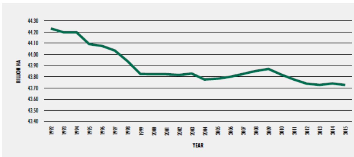
Figure 5. Trends in global tree cover between 1992 and 2015 (FAO and UNEP, 2020)
