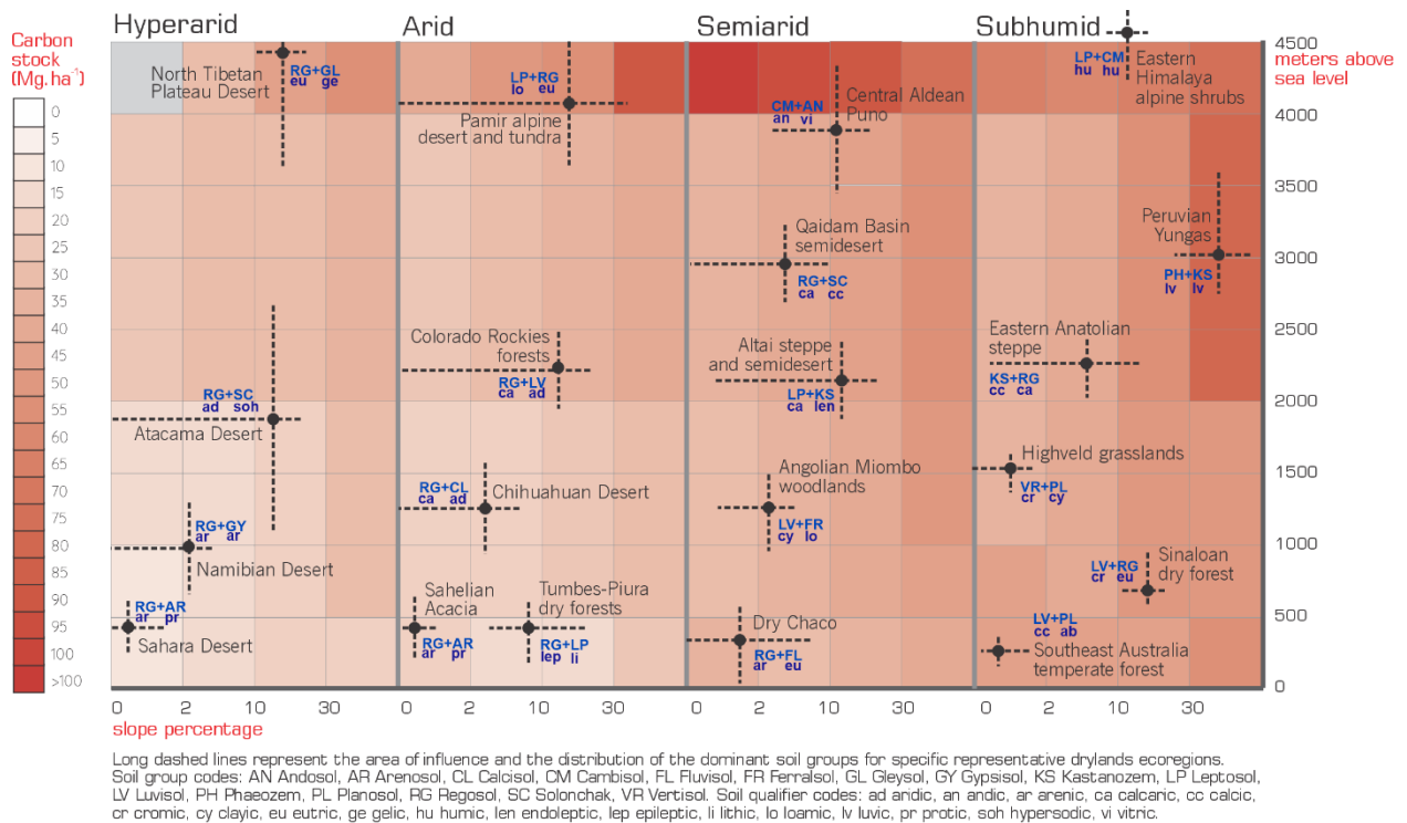
Figure 26. General view of the magnitude and distribution of global SOC stores in drylands (to 30 cm depth)
