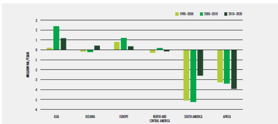
Figure 6. Net forest area change by region between 1990 and 2020 (FAO and UNEP, 2020)
