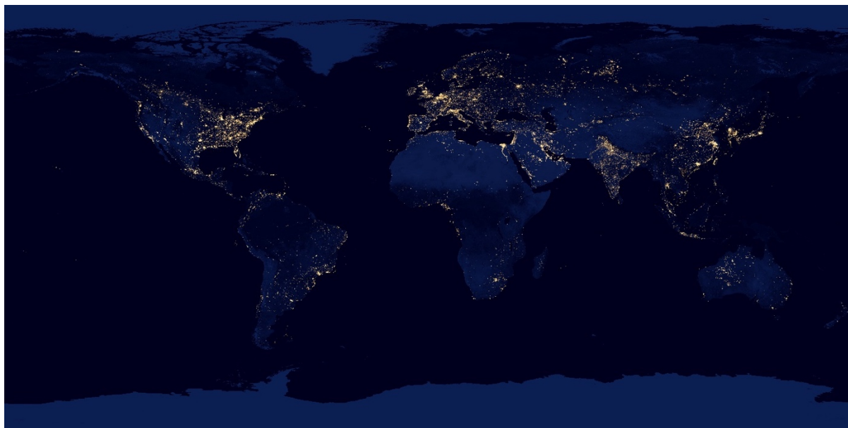
Figure 31. Worldwide image of Earth at night showing the extent of city lights from space, NASA Earth Observatory (NASA, 2012)
