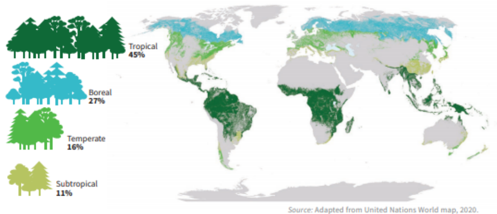
Figure 1. Proportion and distribution of global forest area by climatic domain, 2020 (FAO, 2020b)
