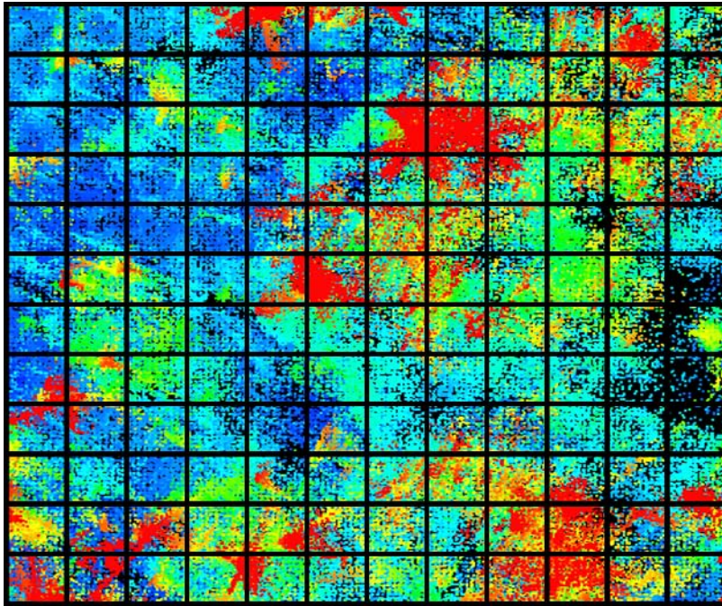
Figure 2 —Example of the spatial grid pattern of field data points and corresponding LIDAR heights (color gradients) within the 4 m x 4 m plot (2D aerial view). Point-intercept data on fuel traits were collected every 0.33 m (cross sections of the grid) throughout the plot.
