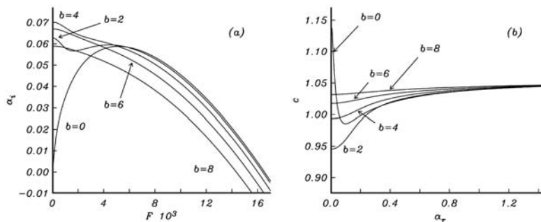
Figure 15 —(a) Amplification curves for varying frequency for 3D disturbances at x = 0.224 ; R_\delta = 150 ; b = 1000 , \beta/R_\delta = for the mildly buoyant flow of U_e = 0.5\text{ m/s} . (b) The corresponding phase speed c variation with wavenumber \alpha_r .
