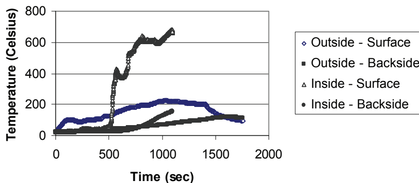
Figure 3—Analytical prediction of dried redwood response to class B brand heat exposure.
