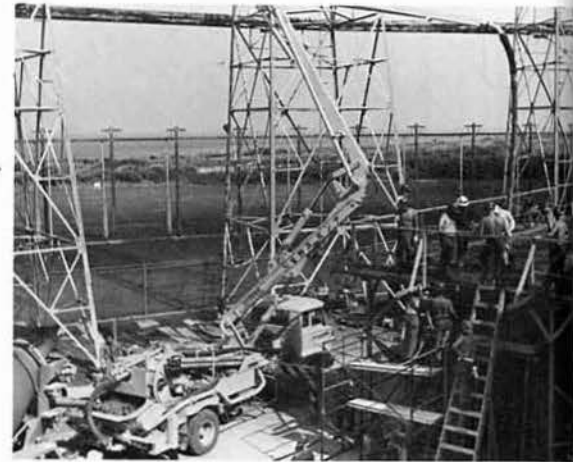
Getting ready to place the concrete roof.
