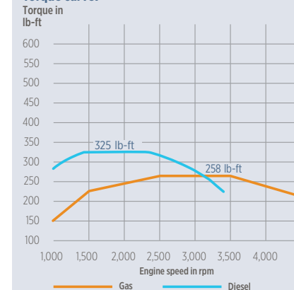
Torque curve:
