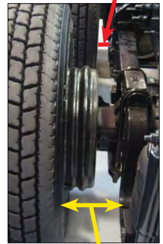
Correct Lateral Clearance
