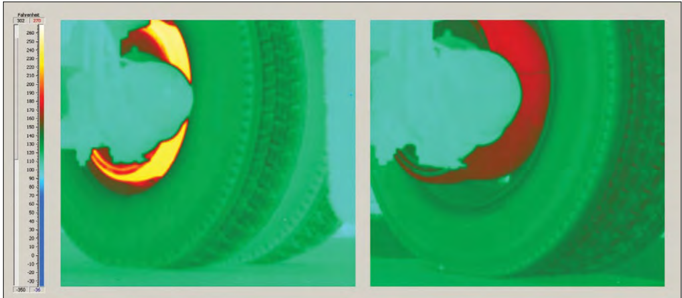
Dual Tires Max temp ~ 215°F
