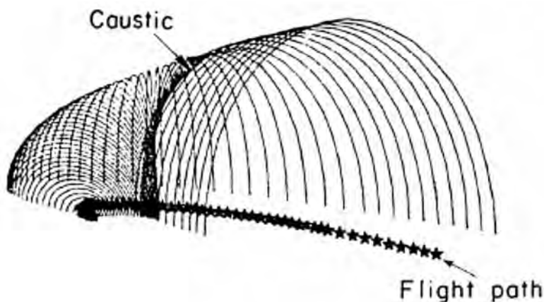
Figure 5. Acoustic wave front above a maneuvering aircraft. NASA.
