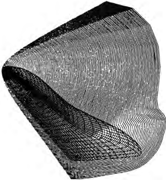
Steady-state three-dimensional shock wave shape, showing the CFD-generated Mach 16.25 flow around a Space Shuttle-like body at a reentry angle of attack of over 39 degrees. From author's collection.
