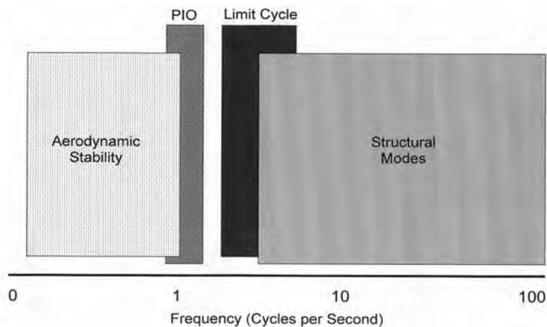
Aircraft frequency spectrum for flight control system design. USAF.
