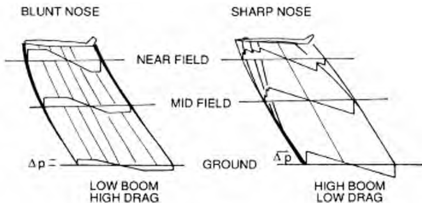
Figure 6. Low-boom/high-drag paradox. NASA.
