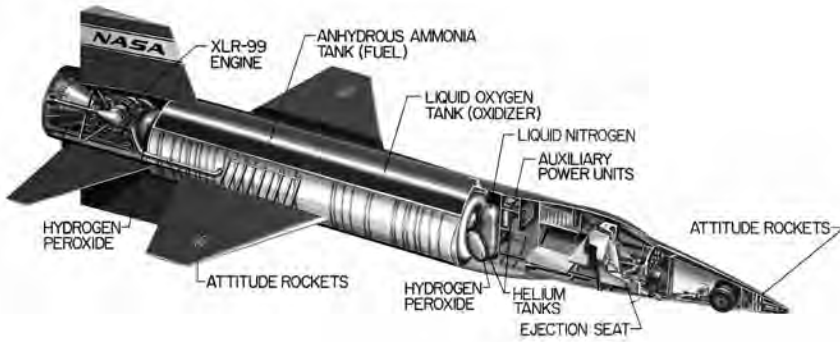
A schematic drawing of the X-15's internal layout. NASA.
