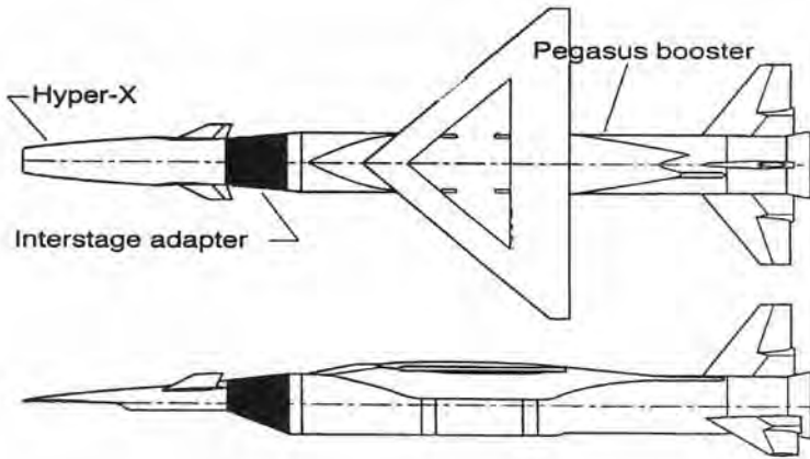
Schematic layout of the Hyper-X (subsequently X-43A) scramjet test vehicle and its Orbital Sciences Pegasus winged booster, itself a hypersonic vehicle. NASA.
