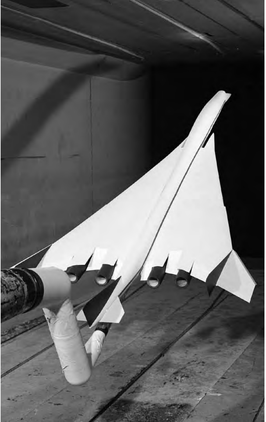
Aerodynamic model of NASA's SCAT-15F supersonic transport design attached for a subsonic wind tunnel test in 1969. NASA.
