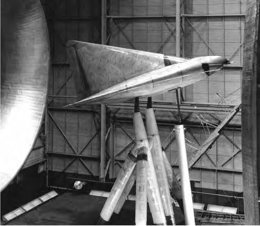
Lippisch DM-1 glider in the Langley Full Scale Tunnel, 1946. The thick-wing section is readily apparent, as is the oversize vertical fin, both of which rendered the concept unsuitable for transonic flight. NASA.
