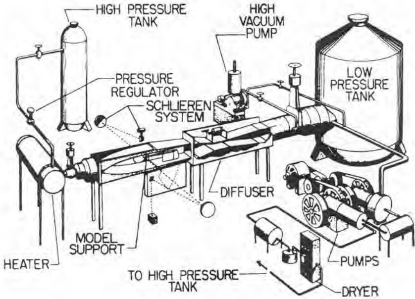
The layout of the Langley 11-inch hypersonic tunnel advocated by John V. Becker. NASA.
