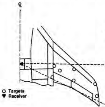
HiMAT Wing with Electro-Optical Deflection Measurement System
