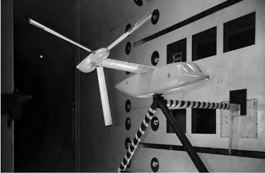
Tilt rotor semi-span dynamic model in the Langley Transonic Dynamics Tunnel. NASA.
