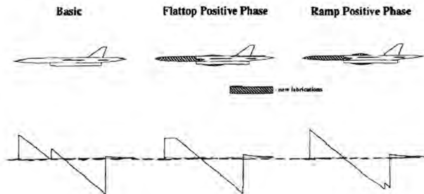
Figure 7. Proposed modifications to BQM-34 Firebee II. NASA.
