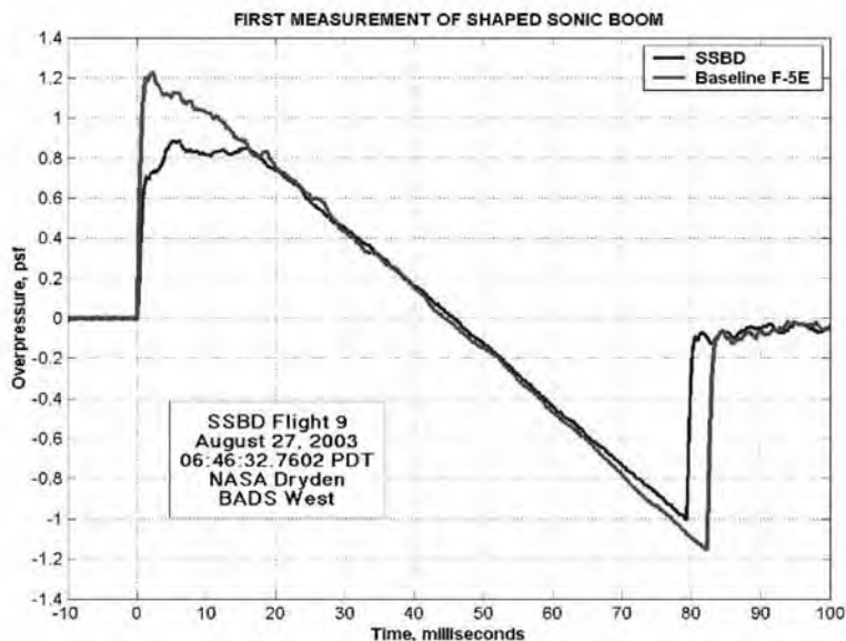
Figure 9. Normal and flattened F-5E sonic boom signatures. NASA.
