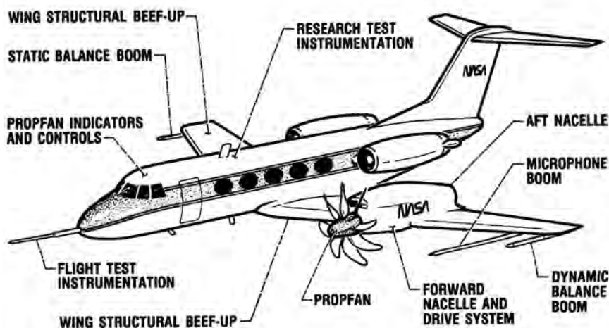
Schematic drawing of the NASA propfan testbed, showing modifications and features proposed for the basic Grumman Gulfstream airframe. NASA.
