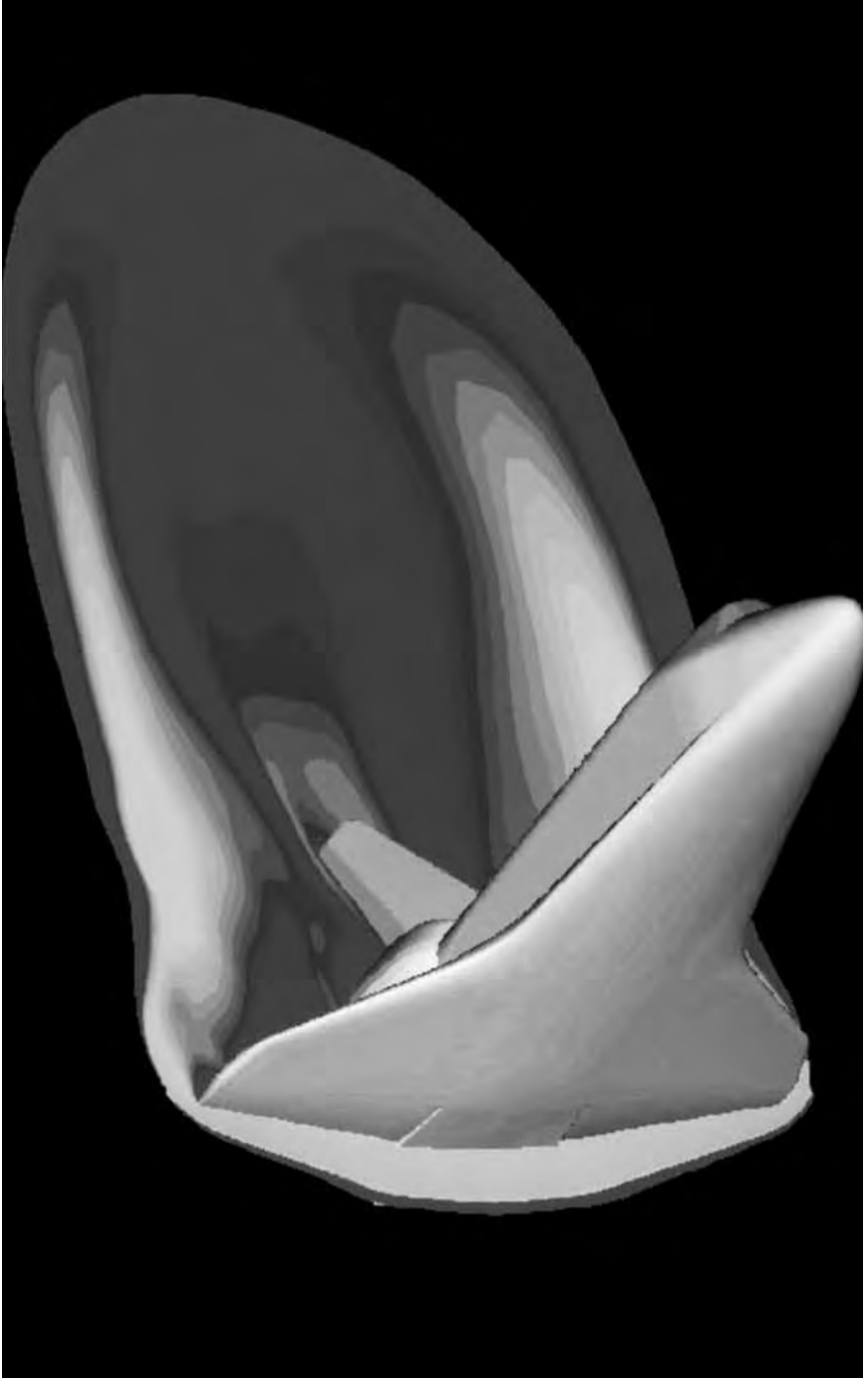
Langley CFD Shuttle study, showing the hypersonic flow pattern as it executes atmospheric entry from orbit. NASA.
