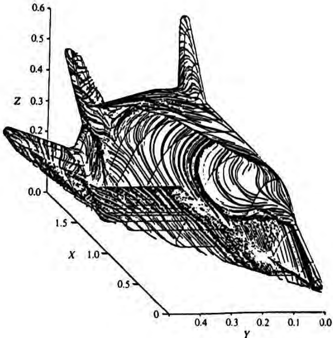
X-24C computed surface streamlines. From author's collection.
