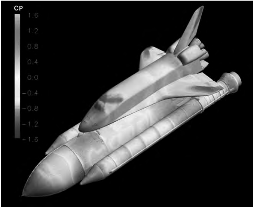
USAF–NASA cooperative CFD Shuttle study. NASA.
