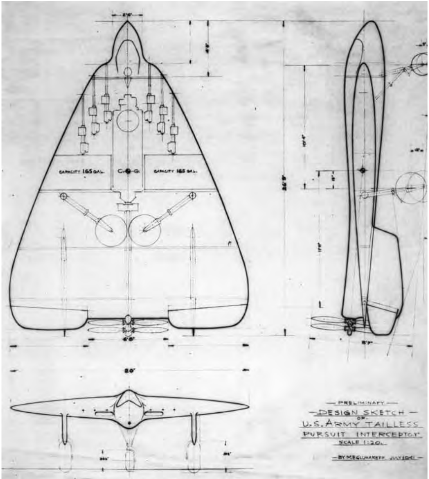
The proposed Gluhareff Dart fighter of 1941, showing both its novel layout and, for the time, nearly as novel tricycle landing gear layout. National Air and Space Museum, Smithsonian Institution.
