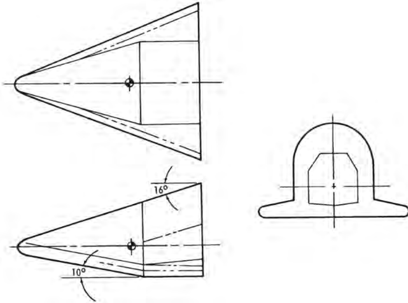
Geometric planform of the McDonnell ASSET reentry test vehicle. USAF.
