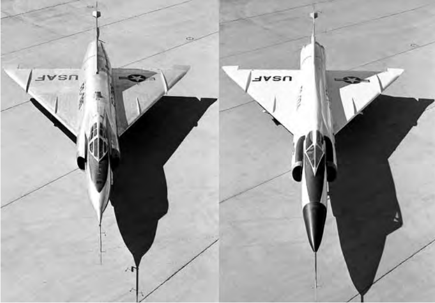
The Air Force's F-102 got a whole new look after implementing Richard Whitcomb's area rule. At left is the YF-102 without the area rule, and at right is the new YF-102A version. NASA.
