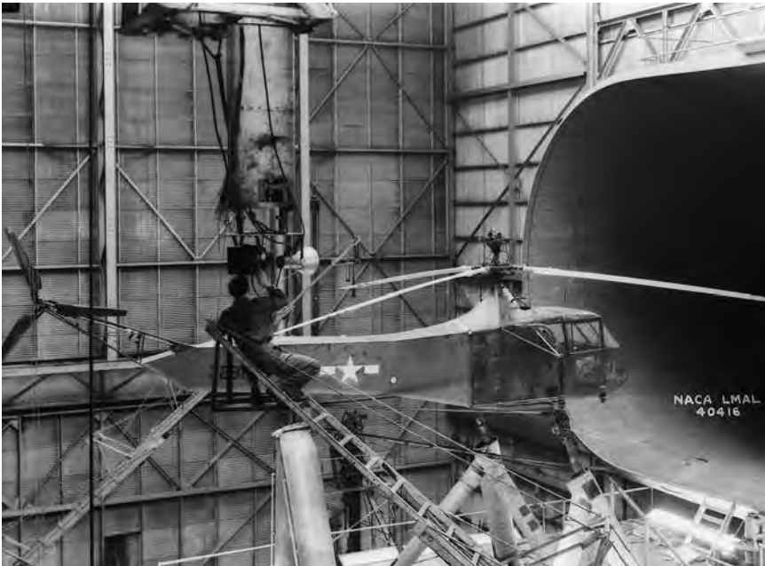
Sikorsky YR-4B tested in the Langley 30 x 60 ft. wind tunnel. NASA.
