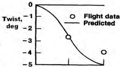
Comparison Flight Data to Prediction (NASTRAN)
