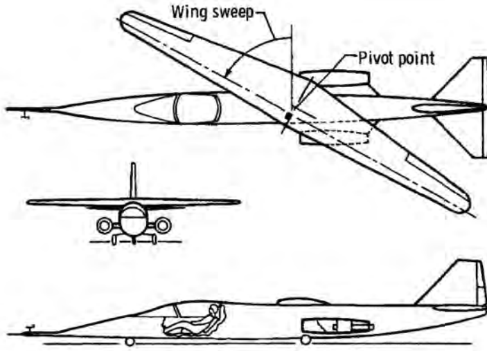
AD-1 three view. NASA.
