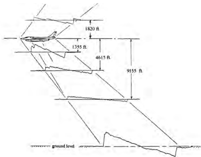
Figure 3. In-flight sonic boom signatures of B-58 at Mach 1.6. USAF.
