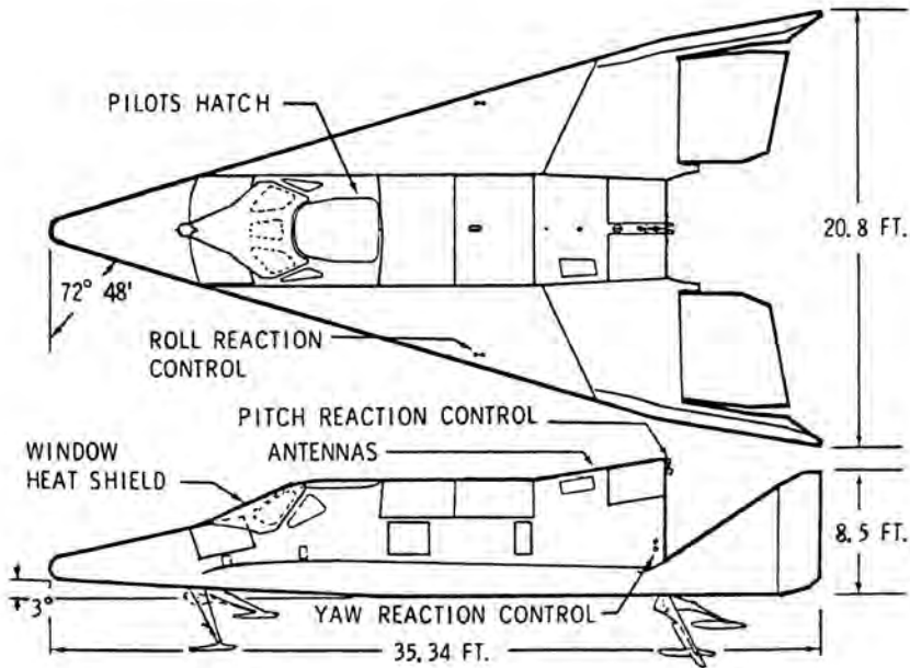
Schematic drawing of the Boeing X-20A Dyna-Soar. USAF.
