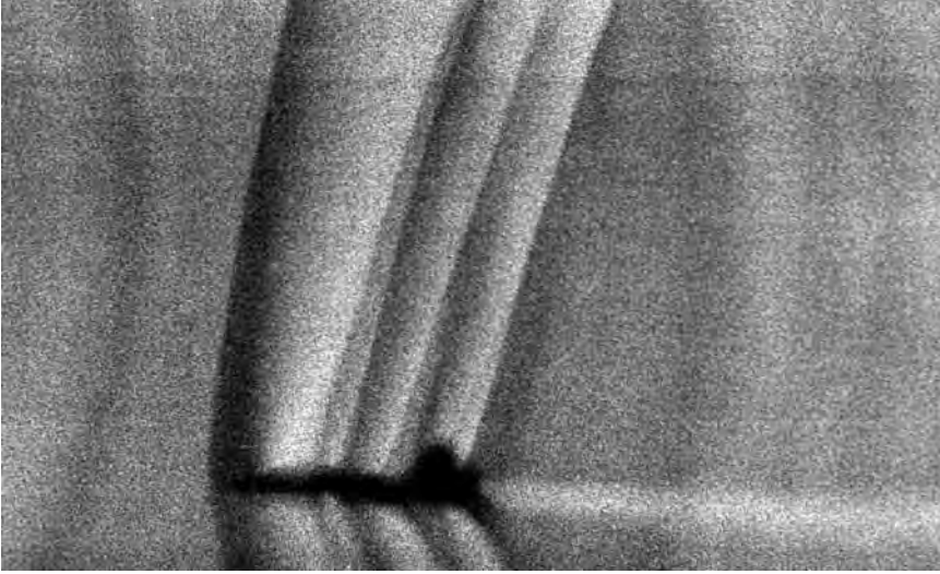
Leonard Weinstein's innovative schlieren photograph showing shock waves emanating from a T-38 flying Mach 1.1 at 13,000 feet, December 1993. NASA.
