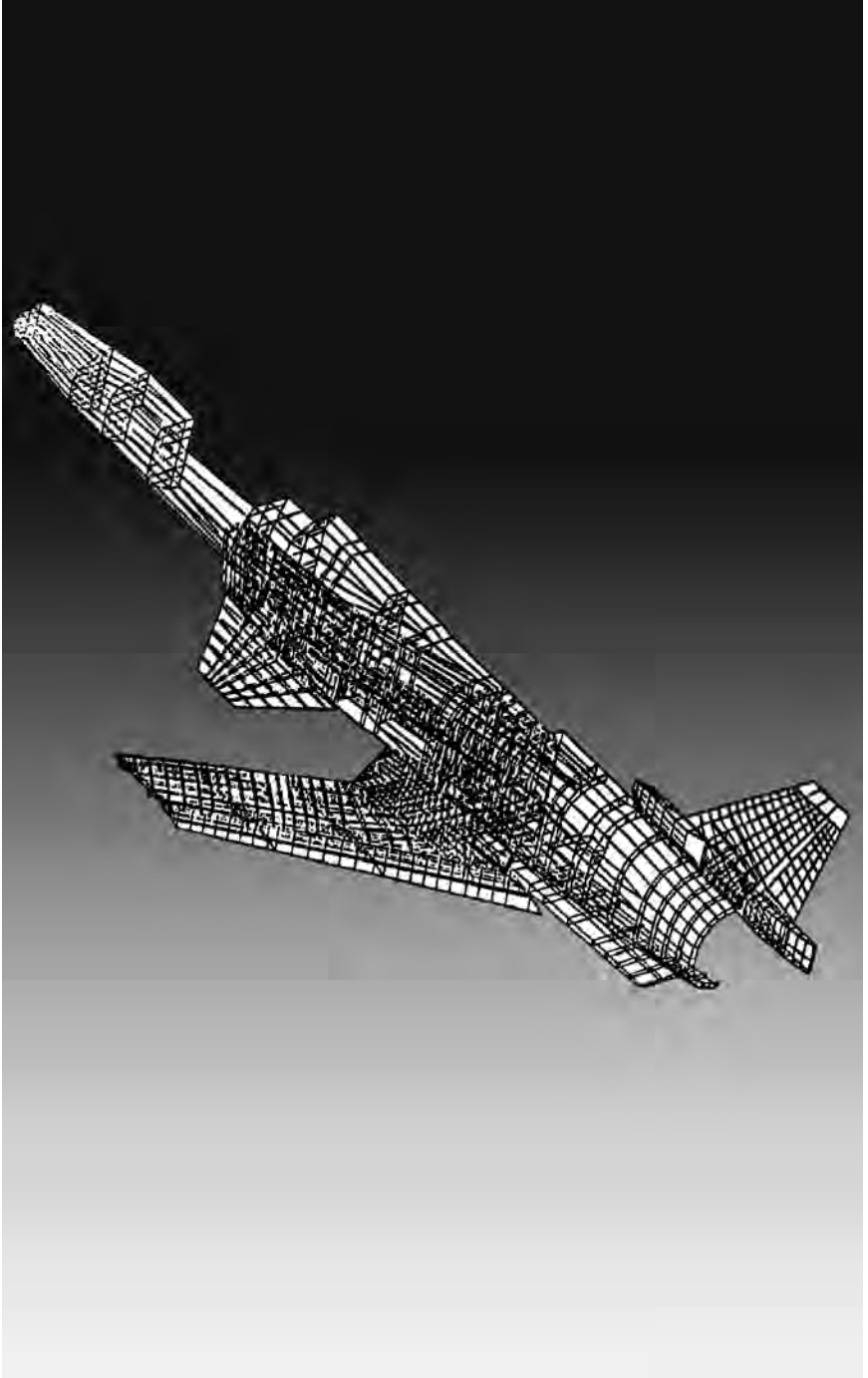
NASTRAN model of the X29A aircraft. NASA.
