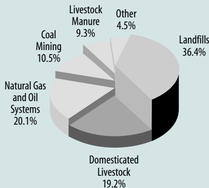
U.S. Methane Emissions From Principal Anthropogenic Sources (1996)
