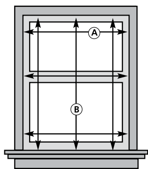
INSIDE MOUNT (IB) Honeycomb Shade
