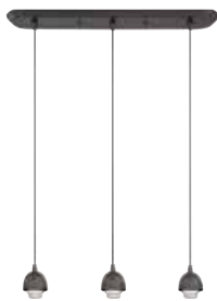
63013 3 Light Mini Pendant Oil Rubbed Bronze Finish Height: 3.50" Width: 23.50" Depth: 4.50" Adjustable Cord: 50" Use (3) Medium (E26) Base Lamps, 60 Watt Maximum
