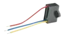
77091 Fan Capacitor 3 MFD and 6.5 MFD 3-Wire 150V
