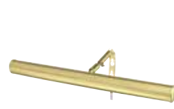
75051 14" Picture Light Polished Brass Finish Height: 4.00" Width: 14.50" Extends: 6.00" Adjustable Cord: 96" Includes (2) T6, 15 Watt Frost Lamps (WL Lamp #03723)
