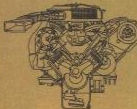
5.0 LITER V8 (305 CUBIC INCH) Short-stroke, valve-in-head design with a Dualjet carburetor.
