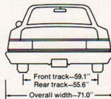
Plymouth Valiant 4-Door Sedan
