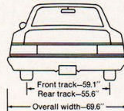
Plymouth Scamp 2-Door Hardtop
