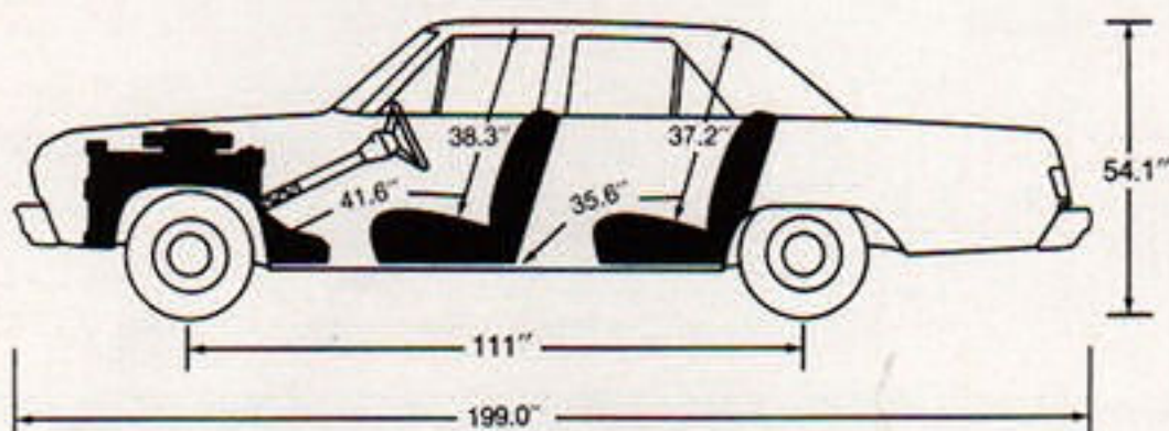
Plymouth Valiant 4-Door Sedan
