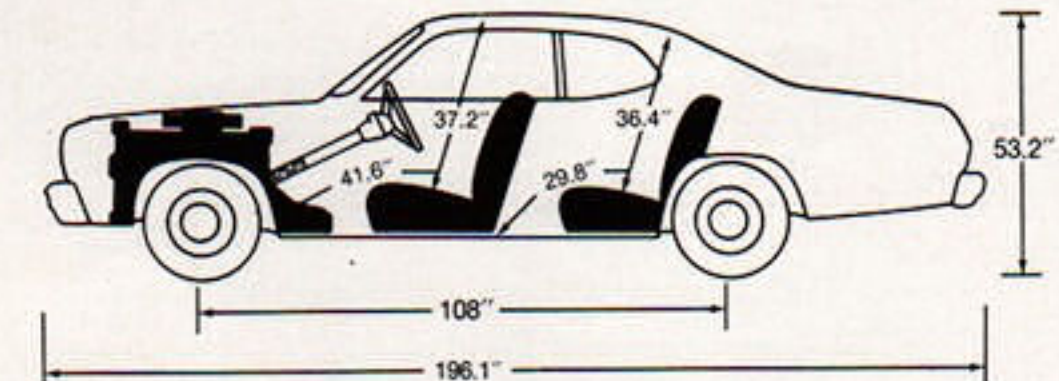
Plymouth Duster 2-Door Coupe
