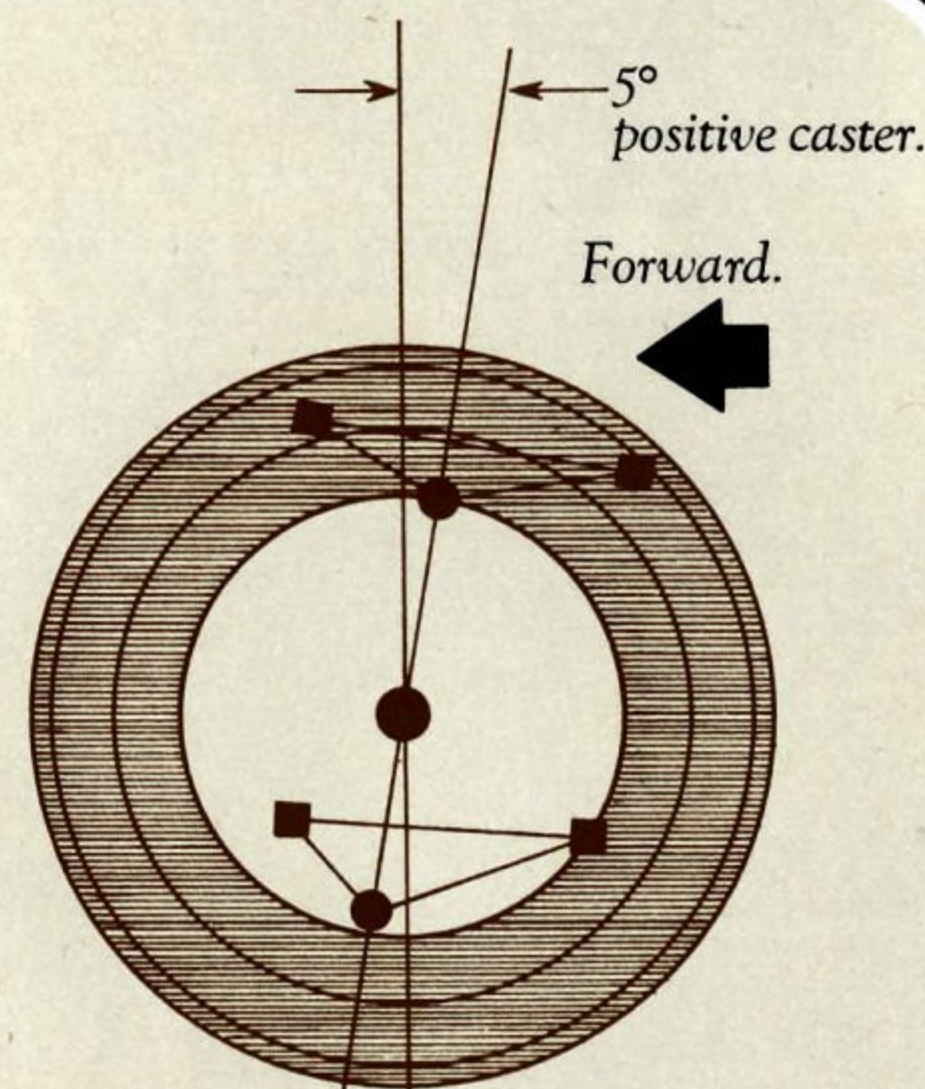
High front caster angle.
