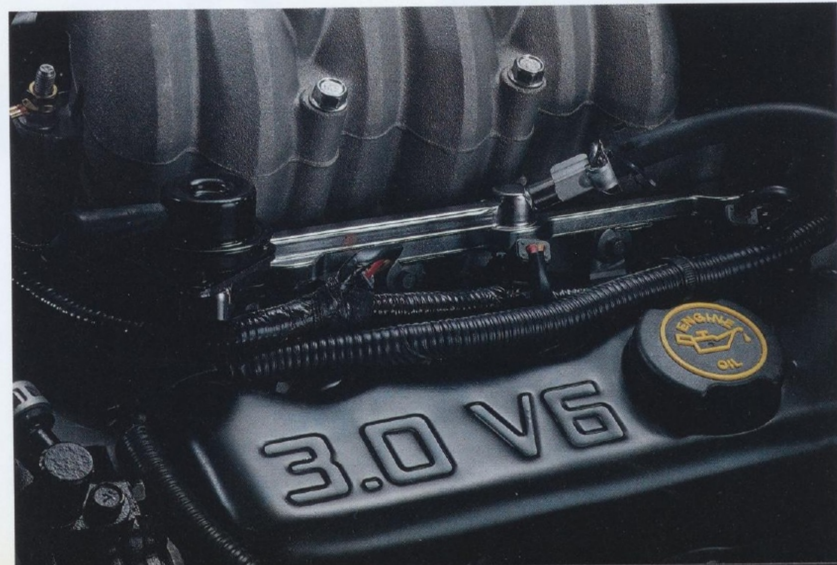
The 3.0L V-6, standard in Probe LX, features 12-in. tuned air intake runners and a multi-port electronic fuel-injection system controlled by the EEC-IV computer.
