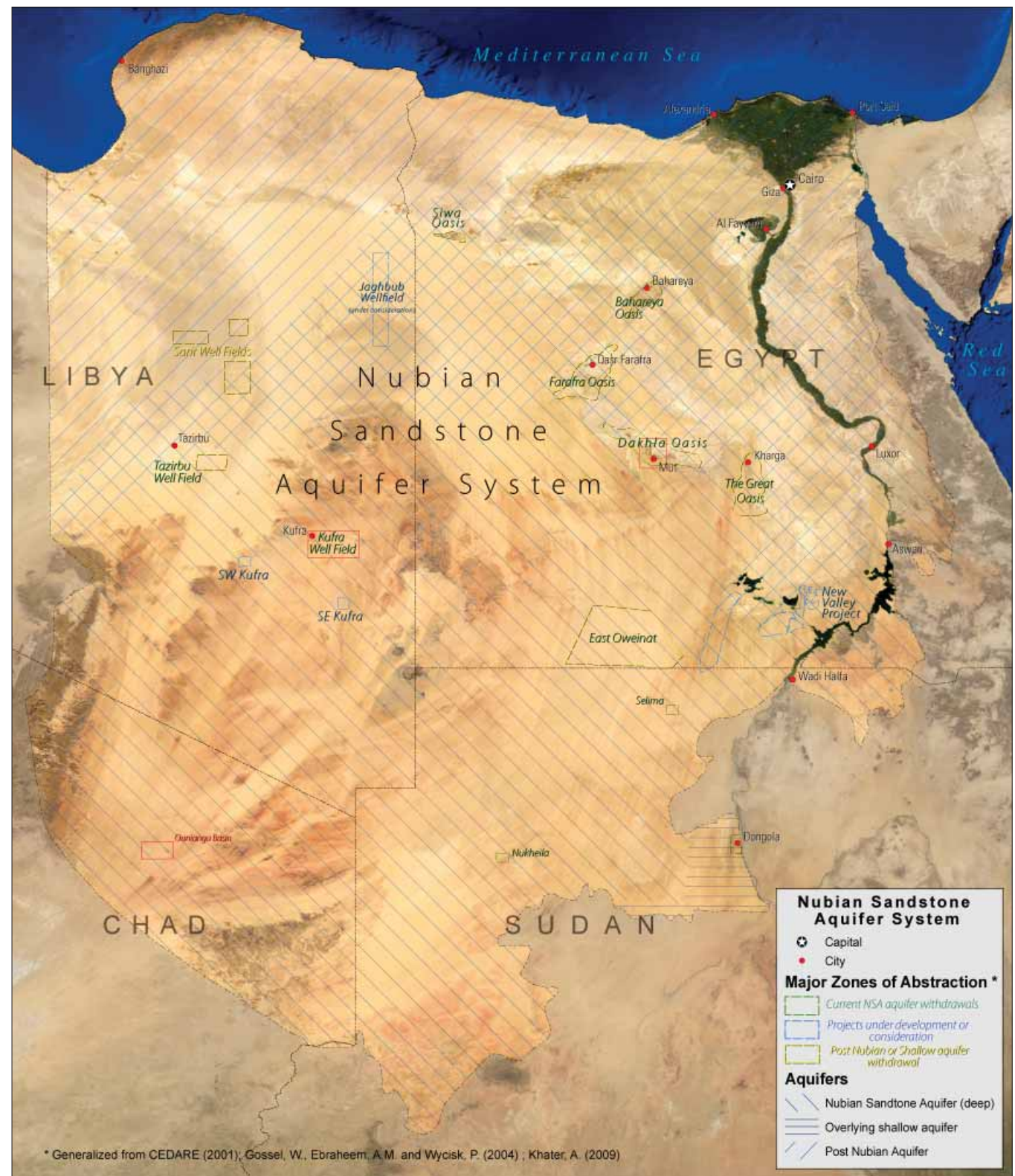
Figure 2.16.1: Nubian Sandstone Aquifer
