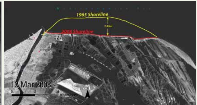
Damietta Promontory, formed by one of the two principle outlets of the Nile River, eroded 1.5 km between 1965 (yellow line) and 2008 (red line)
